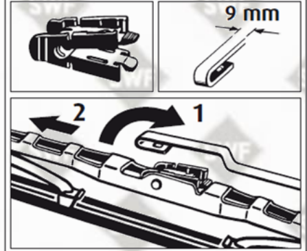
Montage / Fitting T2
