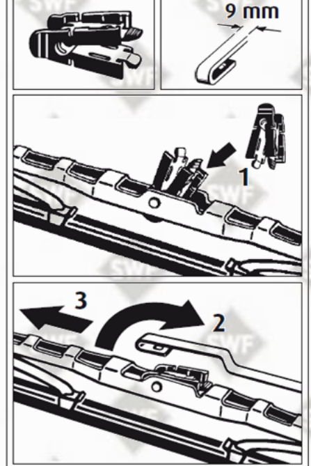
Montage / Fitting T2
