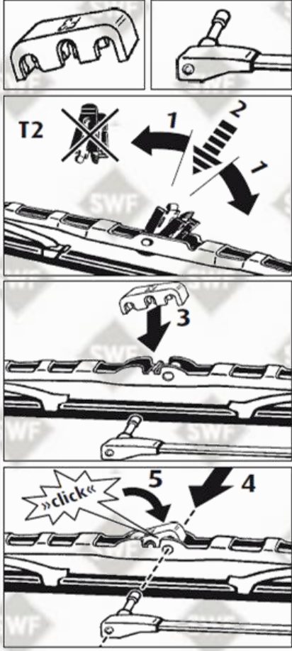
Montage / Fitting F3
